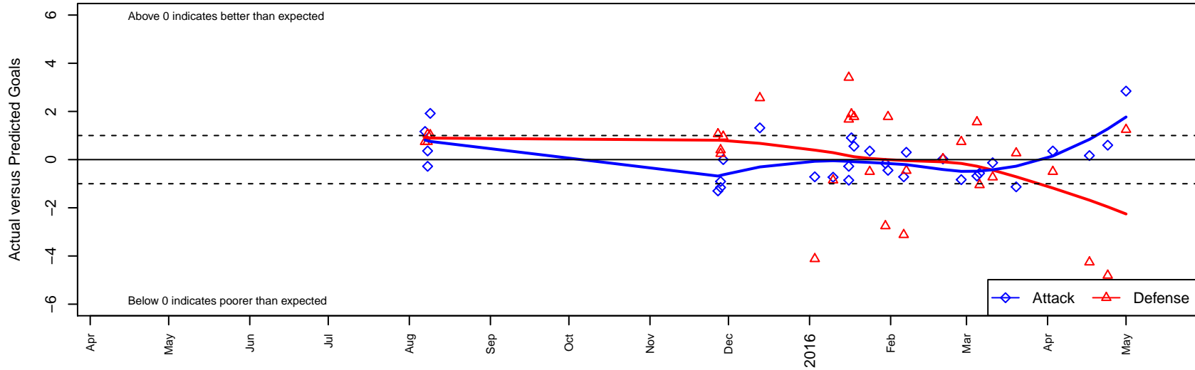
Seattle United Tango G97 Dots are actual minus expected GF (blue circles) and GA (red triangles). Blue line is smoothed change in attack strength. Red is smoothed change in defense strength.
